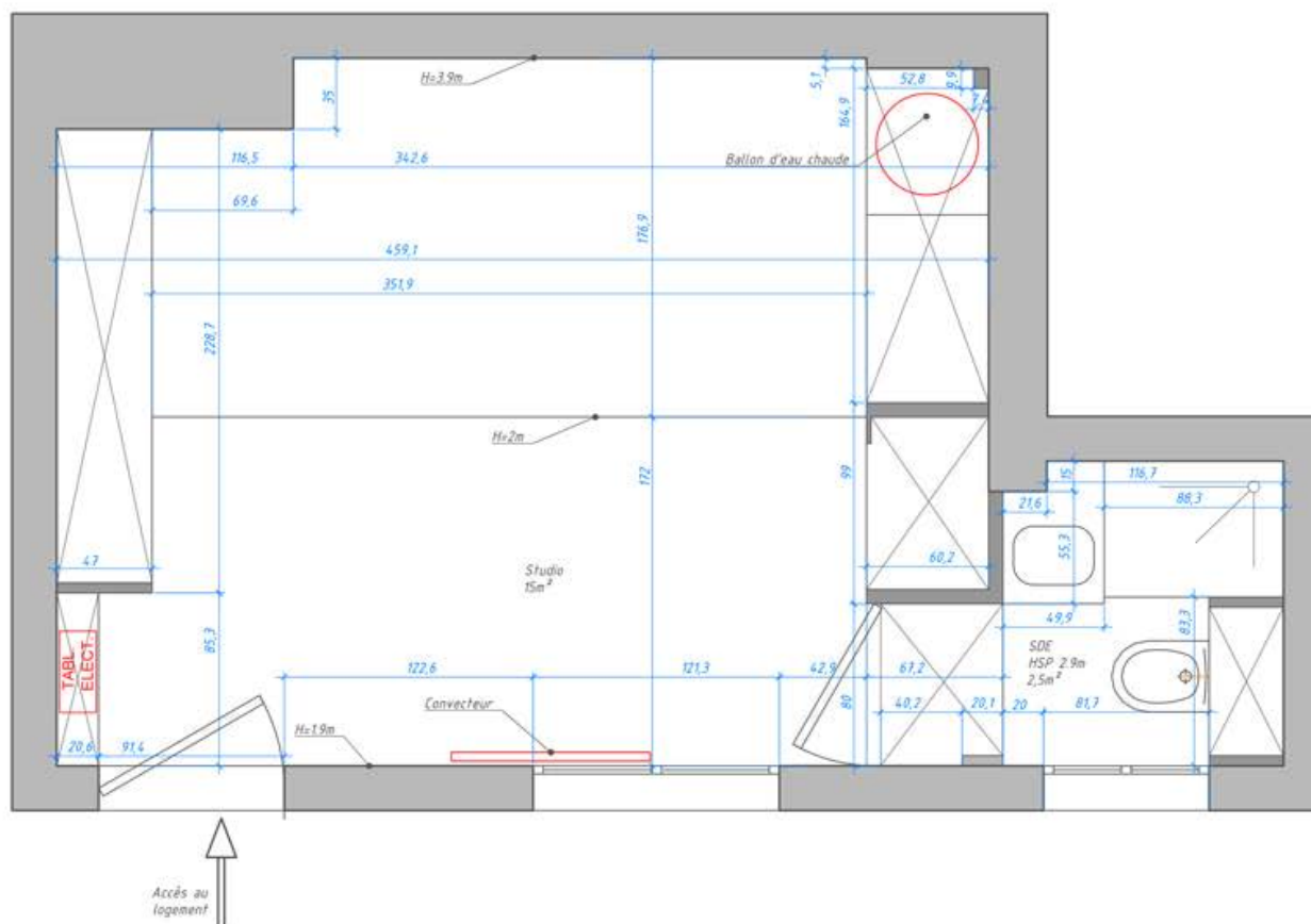
Plan existant
