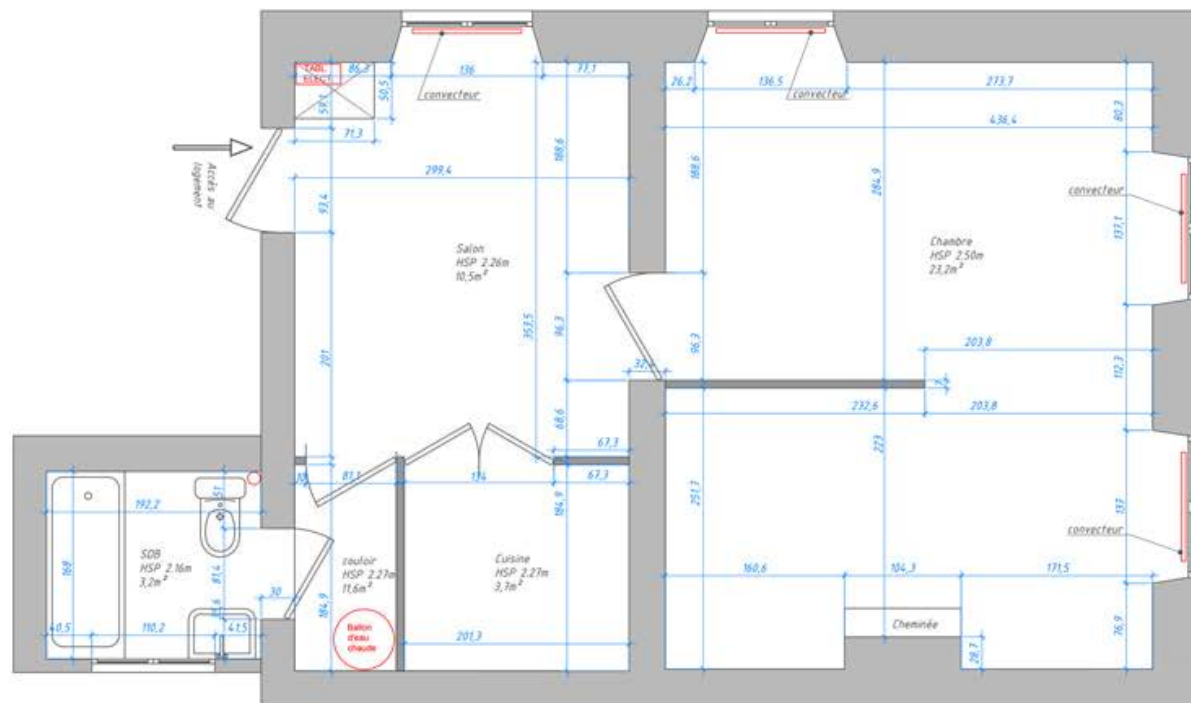
Plan existant
