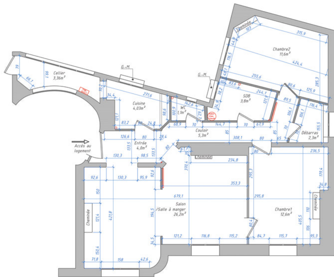
Plan existant
