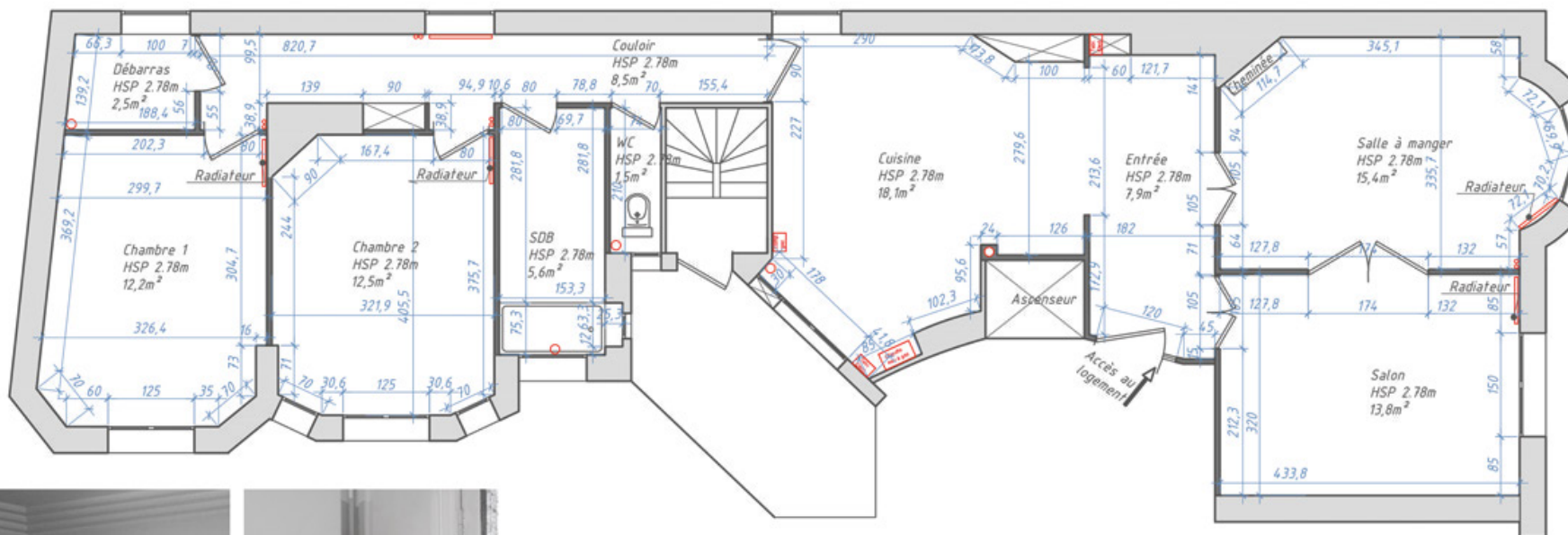
Plan existant
