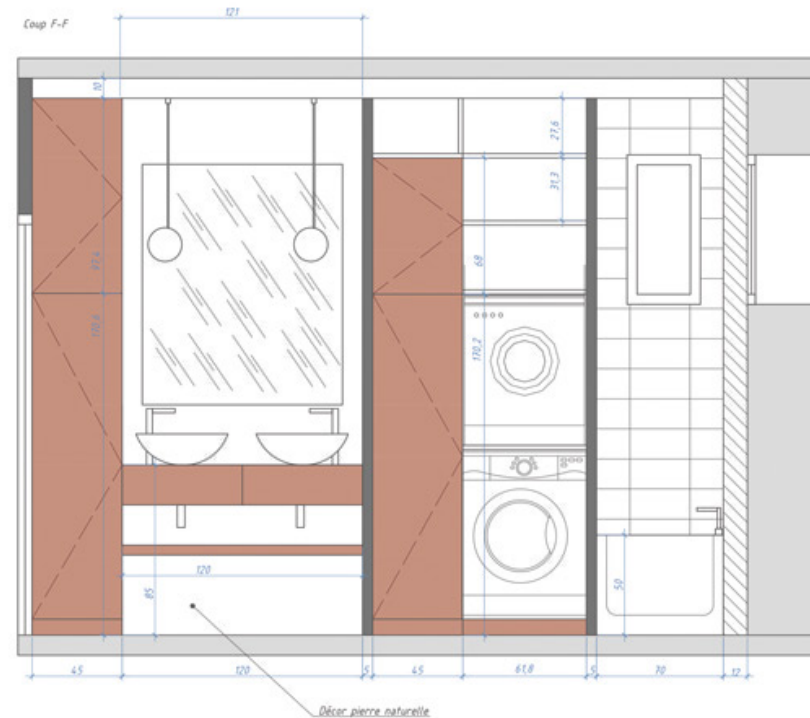
Coup SDB/SDE
