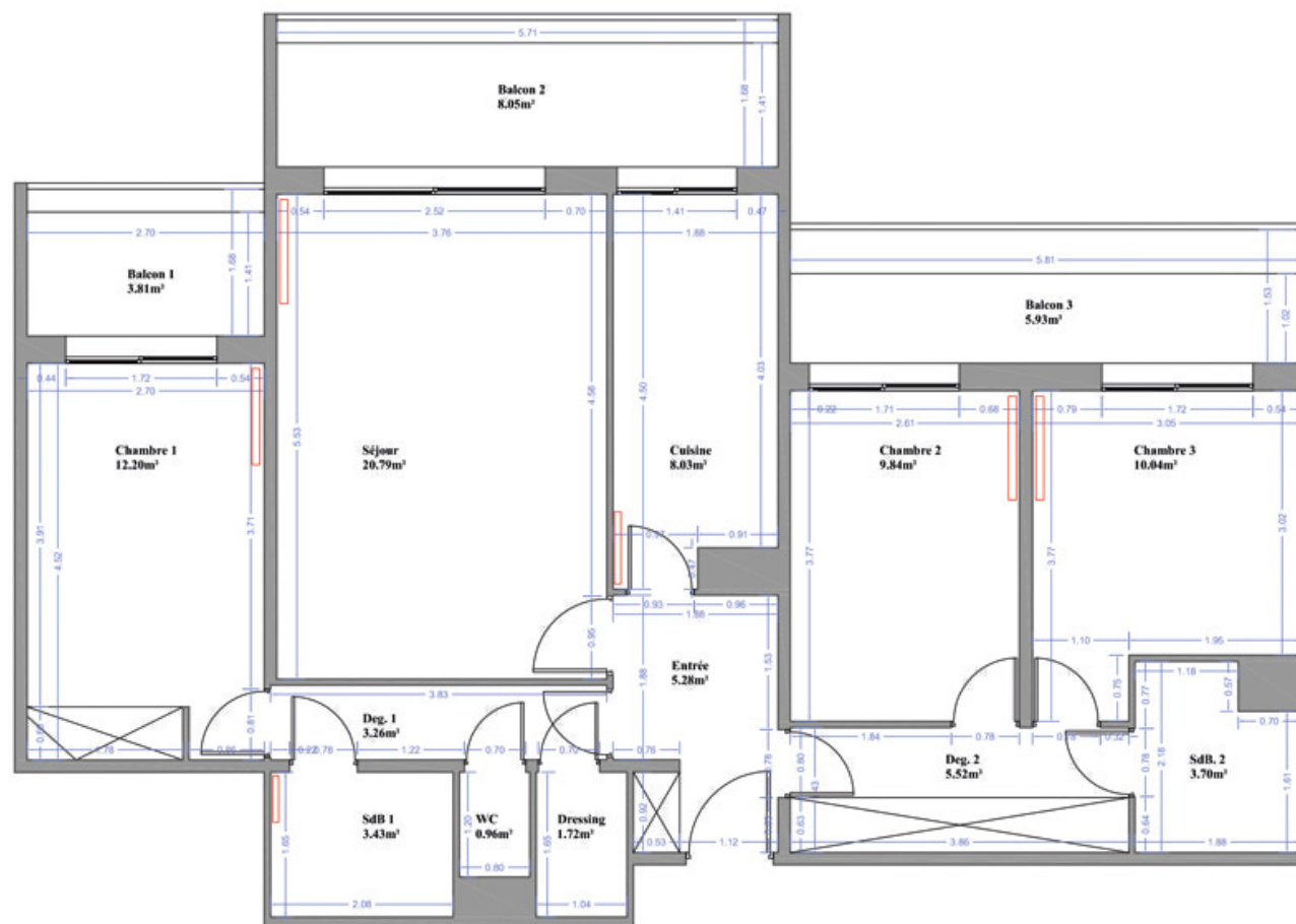
Plan existant
