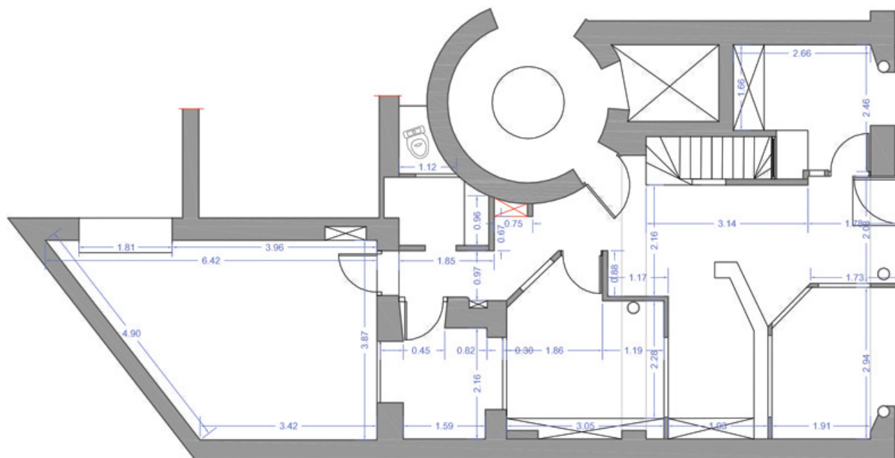
Plan existant
