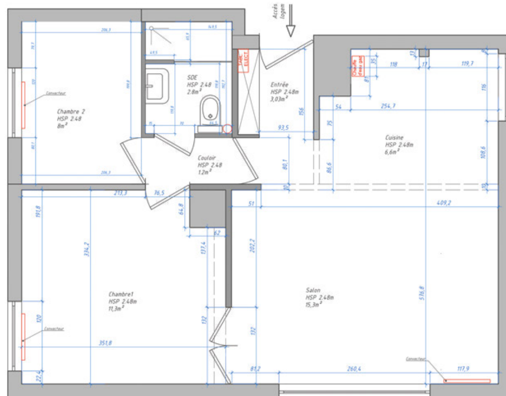
Plan existant
