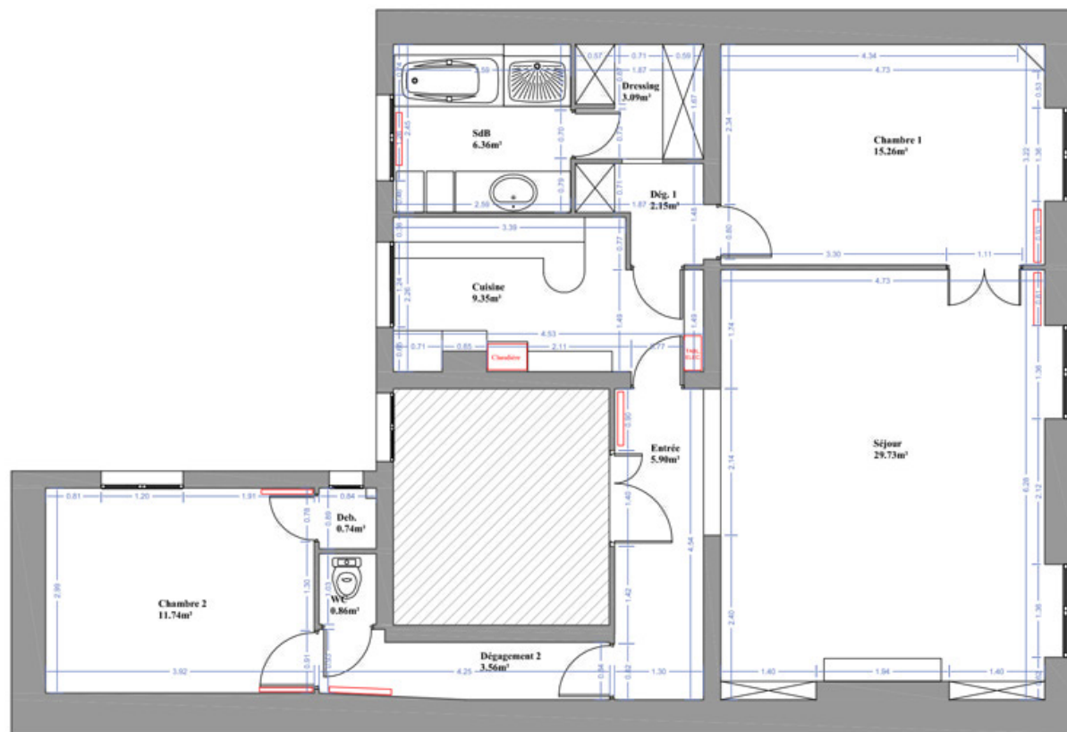
Plan existant
