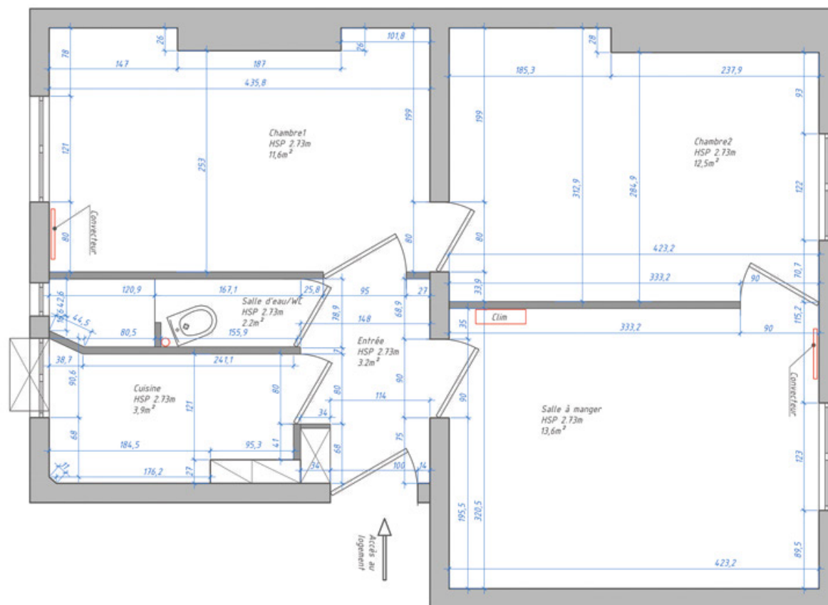
Plan existant
